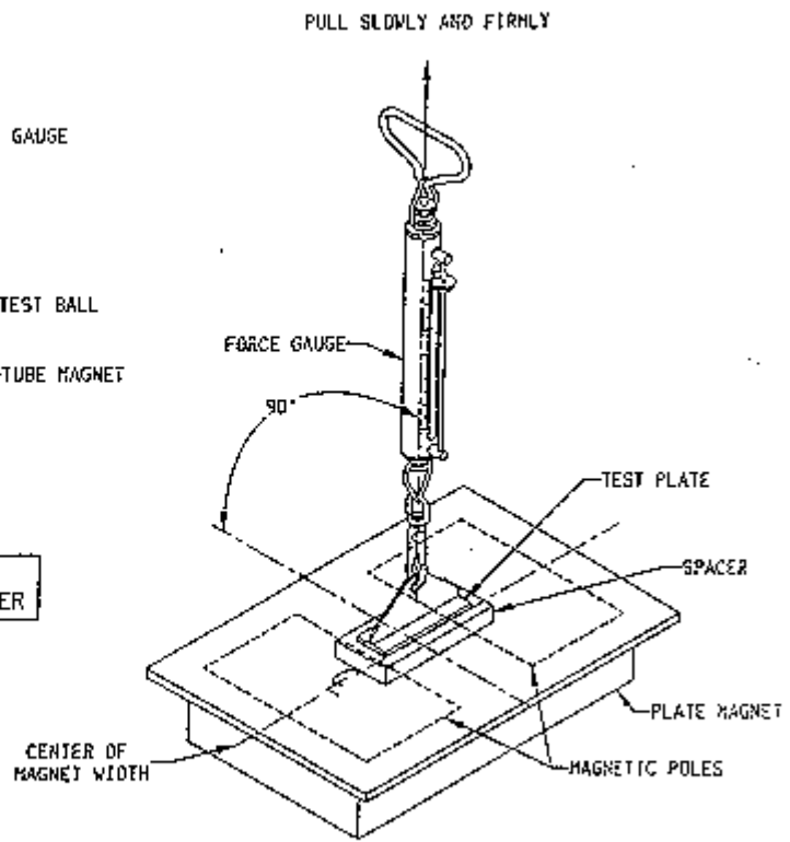
PULL TEST ON PLATE MAGNET WITH TEST PLATE AND SPACER
